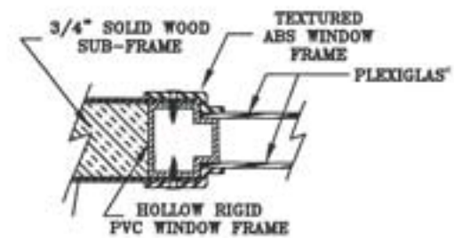
VIEW C-C SHOWING THE WINDOW INSTALLATION
