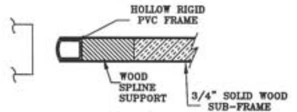
VIEW A-A SHOWING THE JAMB EDGE
