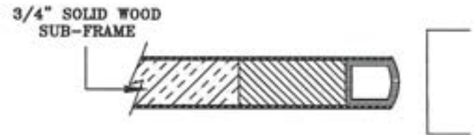
VIEW B-B SHOWING DOOR JAMB EDGE
