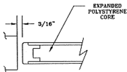
SECTION A-A SHOWING EDGE CHANNEL AT THE DOOR JAMB
